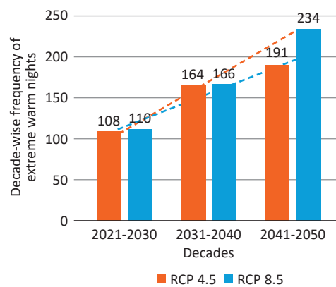
b) Decade-wise projections of extreme warm nights up to 2050
