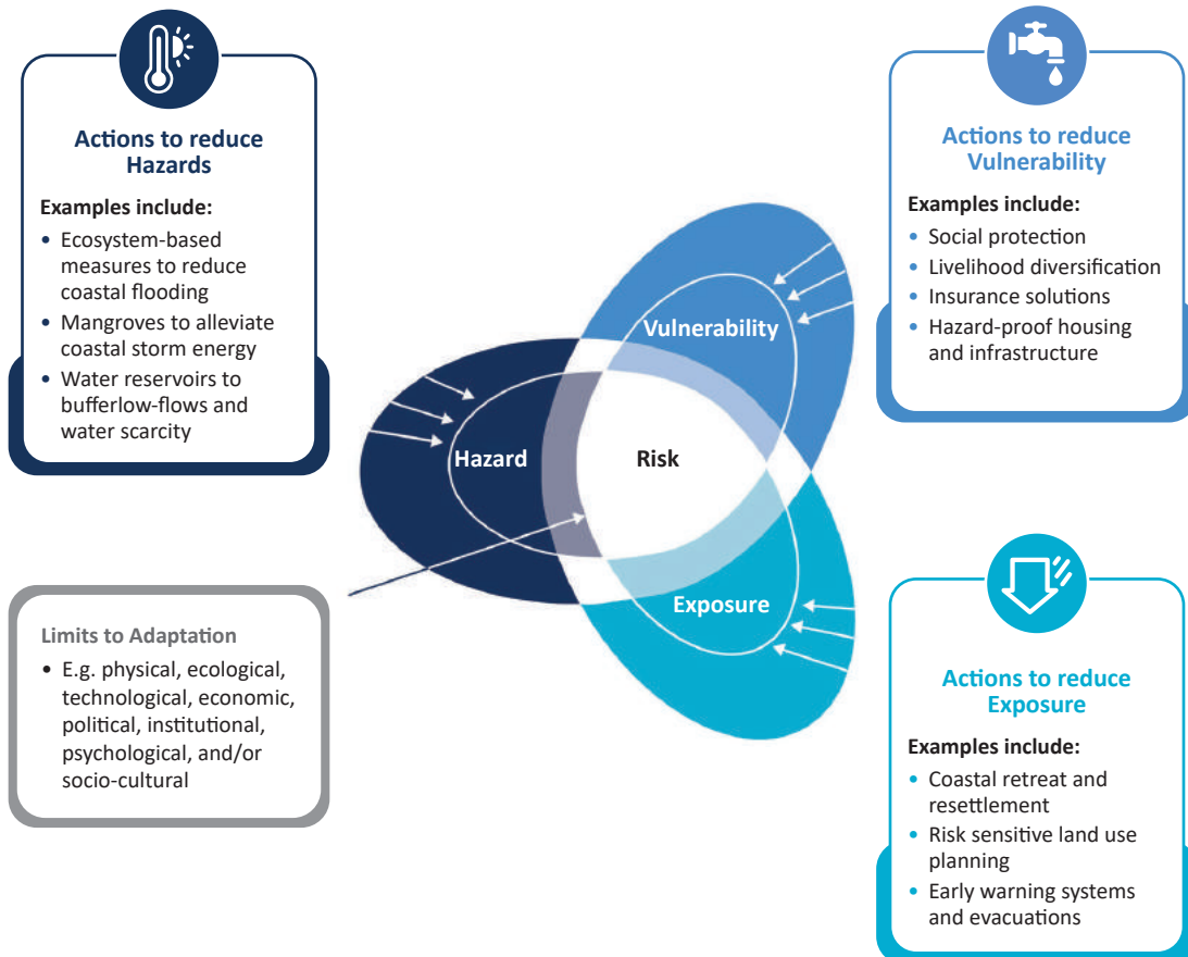
Figure 15: The conceptual framework of the IPCC AR5 risk assessment
