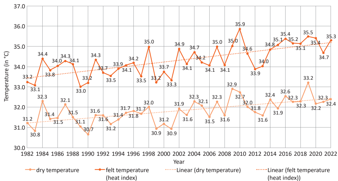
Figure ES3: The difference between dry temperature and felt temperature (dry temperature + relative humidity) has increased by up to 3°C in Thane City over the past 40 years
